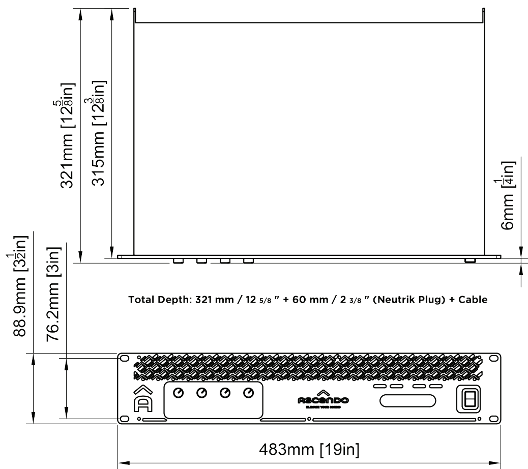
Figure 2. AIA4-2404 dimensions
